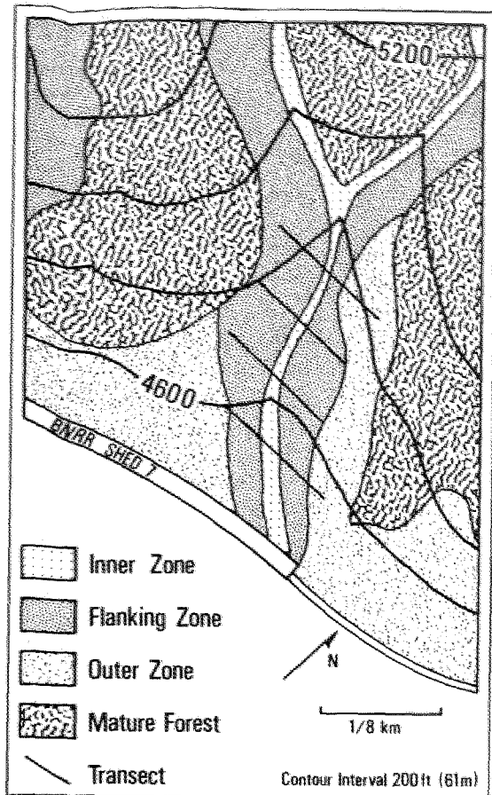
Fig. 1. Map of the vegetative patterns and sample transects on the avalanche path above Shed 7.
