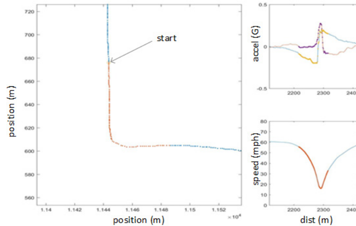
Figure 2. SAX motif with the code: ccbbsbbbbbbaabefffffccecccccccccdeffcaaa
