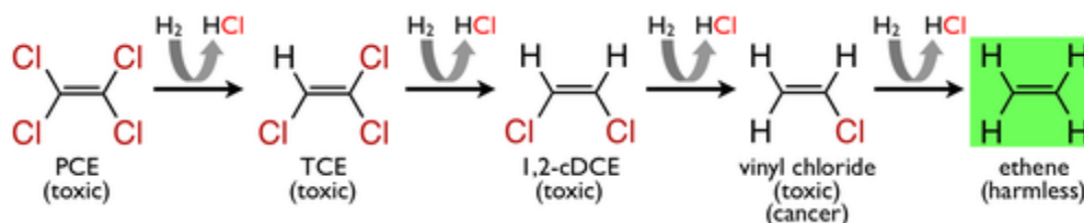
Figure 1: Process of reductive dechlorination of chloroethenes.
