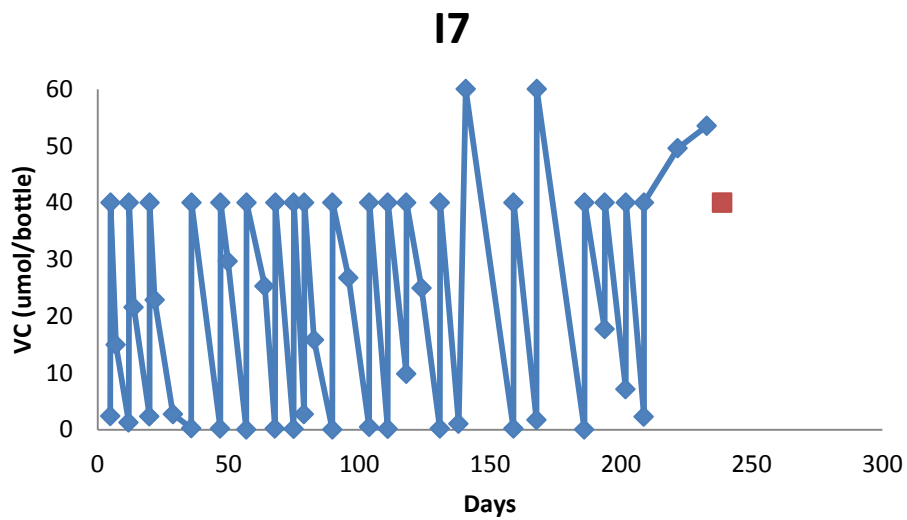
Figure B7. Degradation of VC by isolate 17
