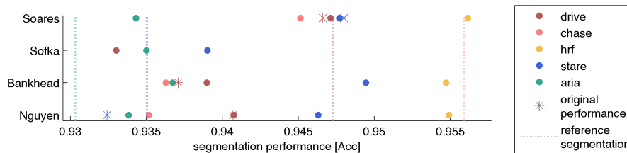
Fig. 1: Comparison of the segmentation performance. The databases are marked with different colors. Solid dots mark the algorithm performance when compared to the ground truth segmentation. Vertical lines mark the performance of second observer when provided. Stars mark the method performance as published in the original papers.
