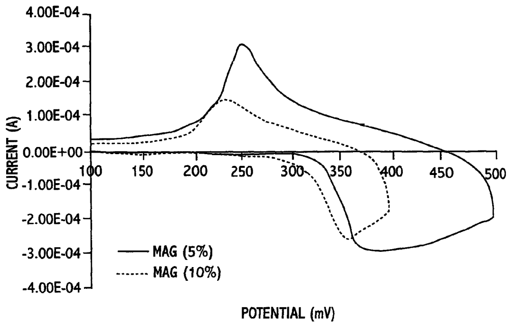
CYCLIC VOLTAMMOGRAMS FOR MAGNETIZED Ni(OH) 2 WITH 5 AND 10 WT% Fe 3 O 4 MIXTURE ELECTRODE AT T=-15°C (v=200mV/SEC)
