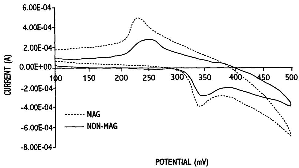
CYCLIC VOLTAMMOGRAMS FOR MAGNETIZED AND NON-MAGNETIZED Ni(OH) 2 / Co(15%) MIXTURE ELECTRODE (v=200mV/SEC)
