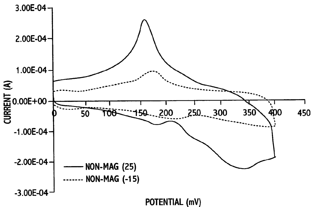
CYCLIC VOLTAMMOGRAMS FOR NON-MAGNETIZED Ni(OH) 2 WITH 5% SmCo MIXTURE ELECTRODE AT T=-15°C (v=200mV/SEC)
