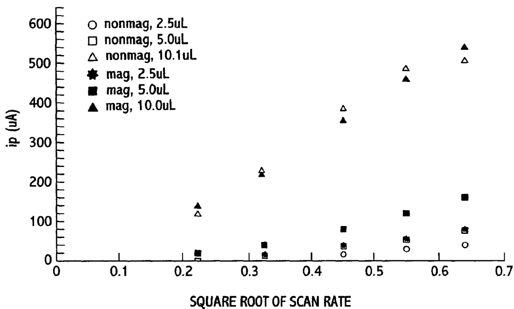
RELATIONSHIP BETWEEN CATHODIC PEAK CURRENT AND THE SQUARE ROOT OF SCAN RATE FOR MAGNETIZED AND NON-MAGNETIZED PURE NICKEL HYDROXIDE ELECTRODE.
