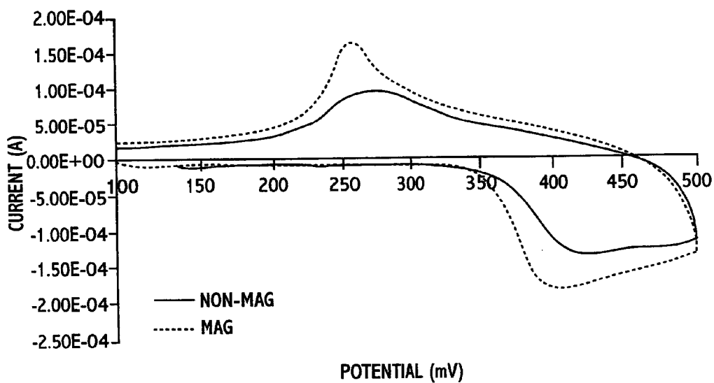
CYCLIC VOLTAMMOGRAMS FOR MAGNETIZED AND NON-MAGNETIZED Ni(OH) 2 / Co(15%) MIXTURE ELECTRODE AT T=-15°C (v=200mV/SEC)
