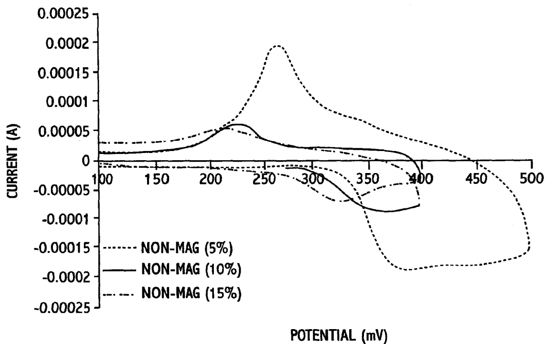
CYCLIC VOLTAMMOGRAMS FOR NON-MAGNETIZED Ni(OH) 2 WITH 5, 10, AND 15 WT% Fe 3 O 4 MIXTURE ELECTRODE AT T=-15°C (v=200mV/SEC)
