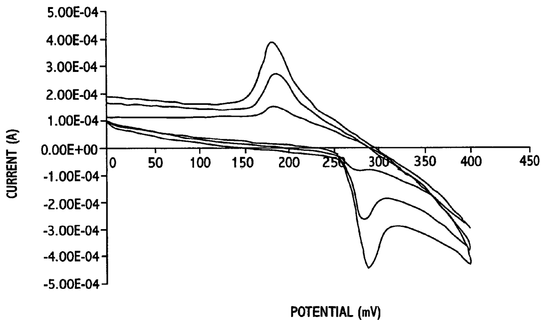
CYCLIC VOLTAMMOGRAMS FOR MAGNETIZED PURE NICKEL HYDROXIDE ELECTRODE AT DIFFERENNT SCAN RATES.
