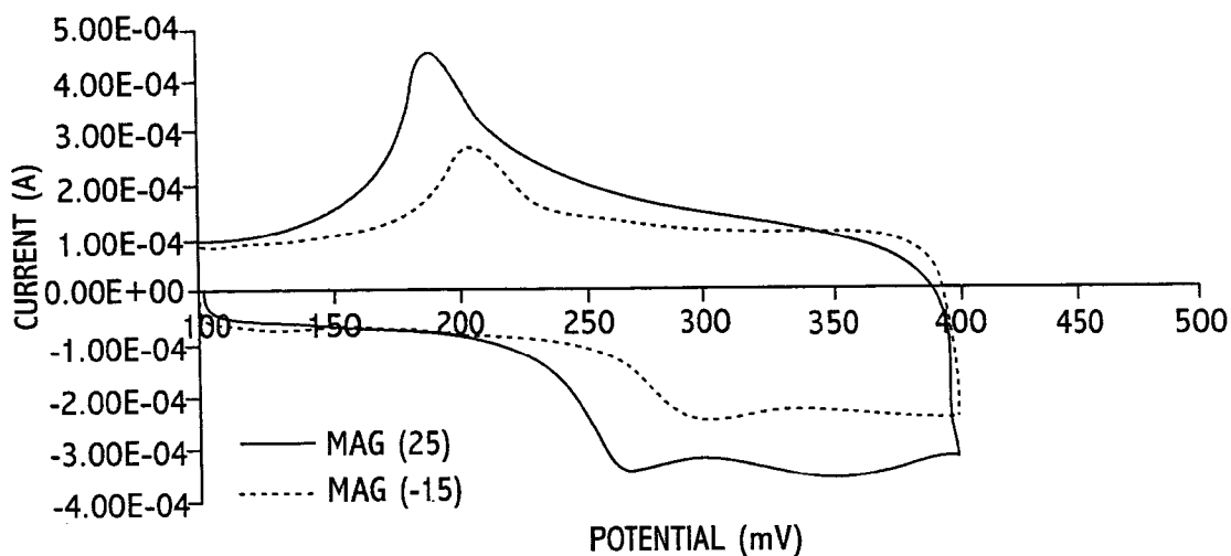
CYCLIC VOLTAMMOGRAMS FOR MAGNETIZED Ni(OH) 2 WITH 5% SmCo MIXTURE ELECTRODE AT T=-15°C (v=200mV/SEC)
