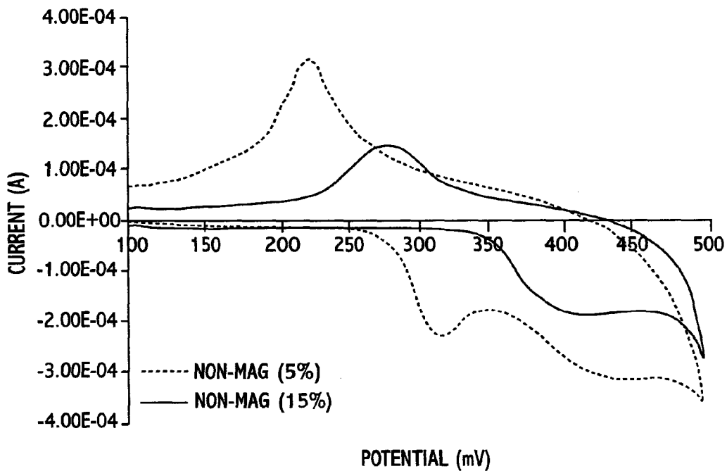
CYCLIC VOLTAMMOGRAMS FOR NON-MAGNETIZED Ni(OH) 2 WITH 5% AND 15% NdFeB MIXTURE ELECTRODE ( \nu=200\text{mV/SEC} )
