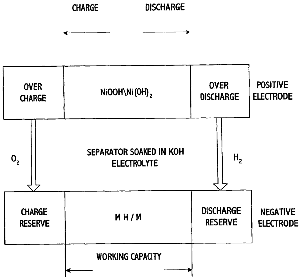
OPERATING PRINCIPLE OF A SEALED Ni-MH CELL
