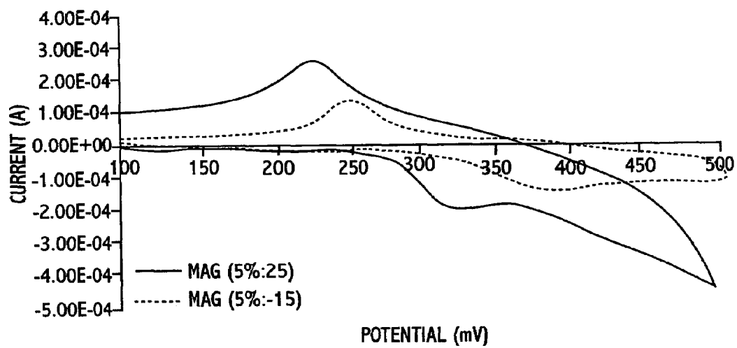
CYCLIC VOLTAMMOGRAMS FOR MAGNETIZED Ni(OH) 2 WITH 5% NdFeB MIXTURE ELECTRODE AT T=-15°C (v=200mV/SEC)
