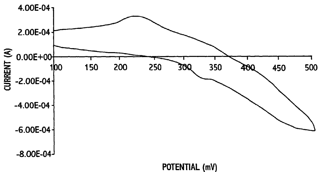
CYCLIC VOLTAMMOGRAMS FOR NON-MAGNETIZED Ni(OH) 2 / GLASS BEADS (5%) MIXTURE ELECTRODE (v=200mV/SEC)
