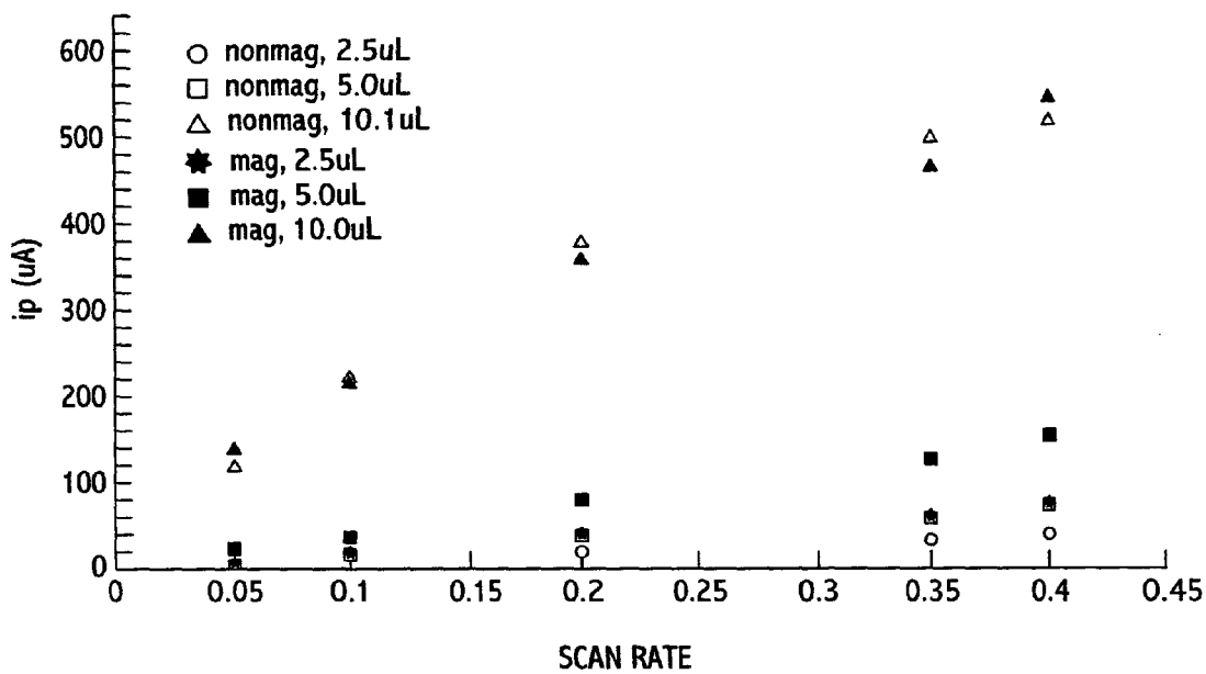
RELATIONSHIP BETWEEN CATHODIC PEAK CURRENT AND SCAN RATE FOR MAGNETIZED AND NON-MAGNETIZED PURE NICKEL HYDROXIDE ELECTRODE.
