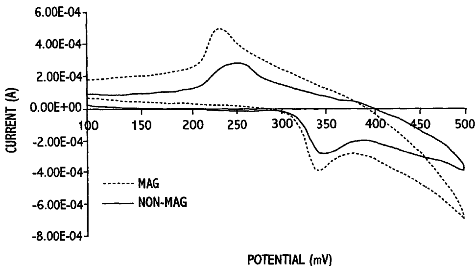
CYCLIC VOLTAMMOGRAMS FOR MAGNETIZED AND NON-MAGNETIZED Ni(OH) 2 / Co(15%) MIXTURE ELECTRODE (v=200mV/SEC)
