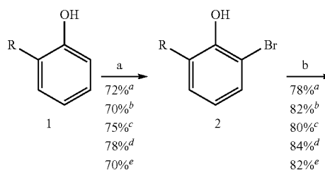
Scheme 1. Synthesis of 4-HTFE phenols.
